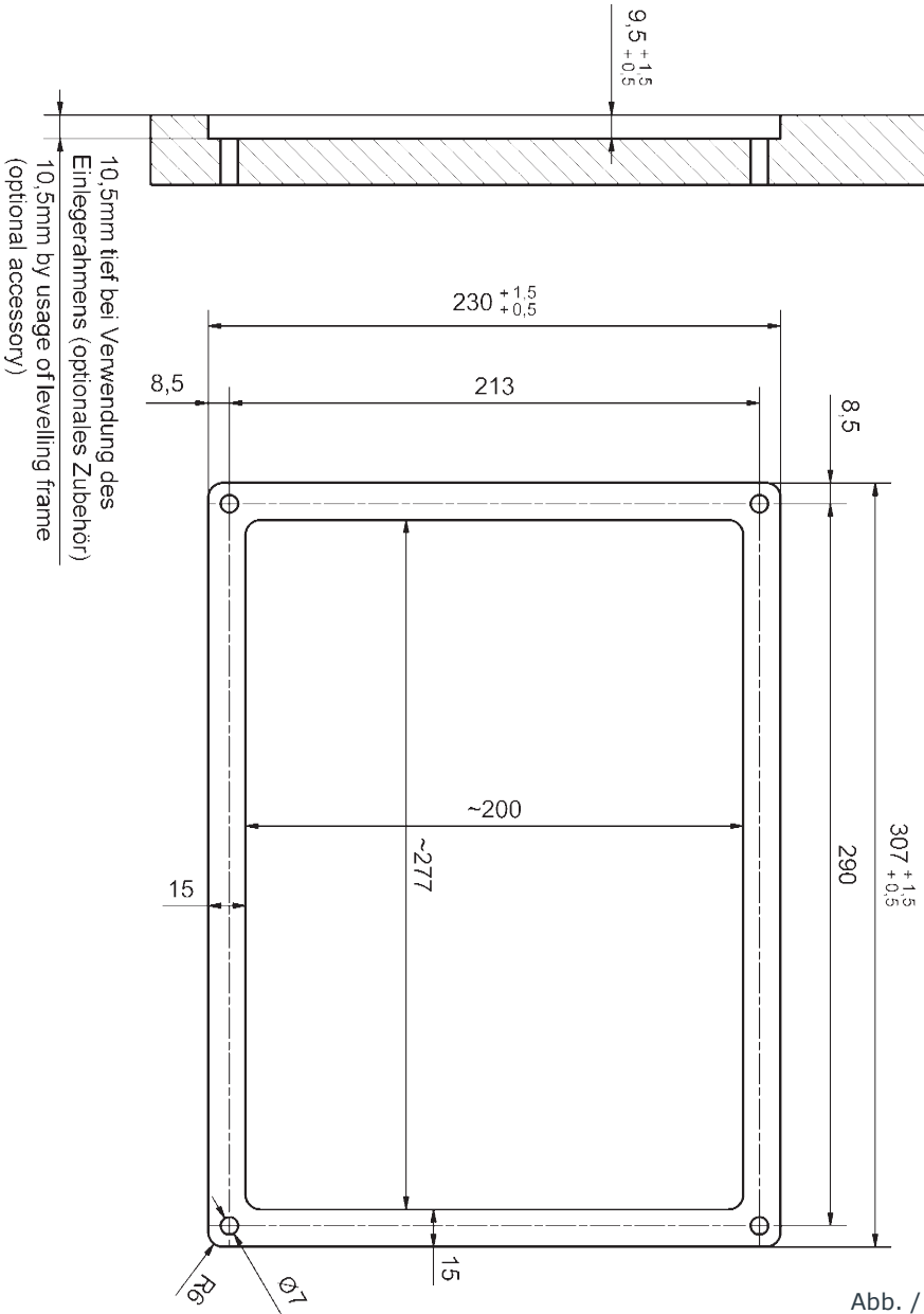
Abb. / Fig. 13 Required installation dimensions on the router table
