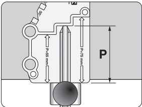
Mount the tool with the same protrusion, P.
