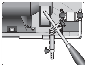
Shape one side at a time and use the whole width of the wheel. Finish with a full swing over the entire bevel.
