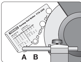
Set the Universal Support. Select hole A or B.
